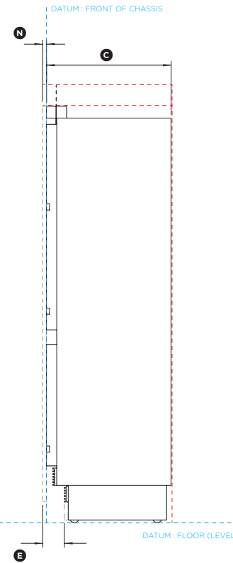
PROFILE VIEW
