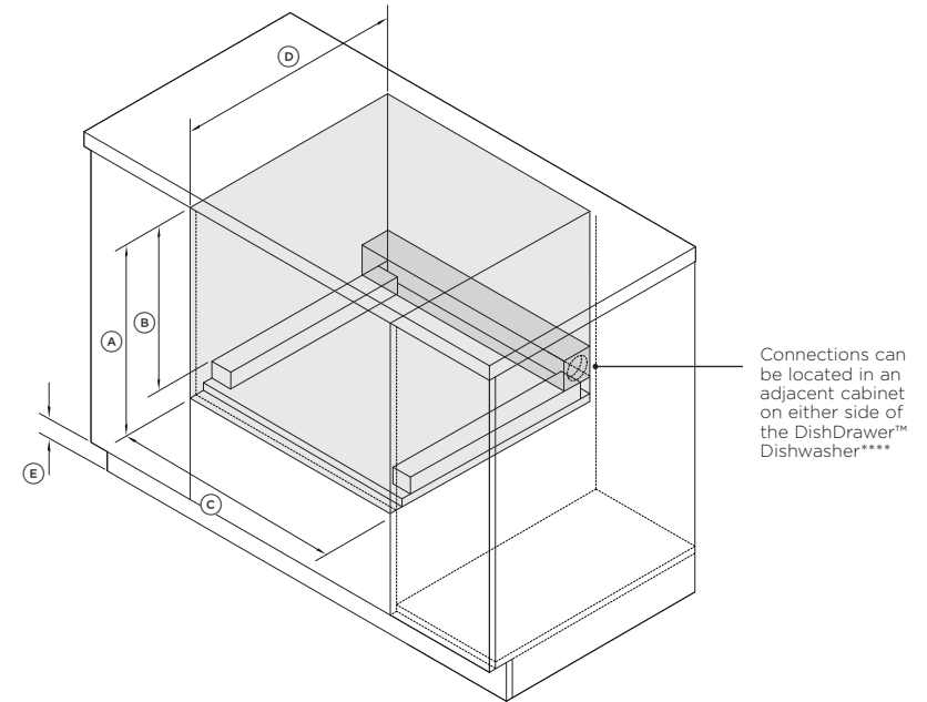
ISOMETRIC
