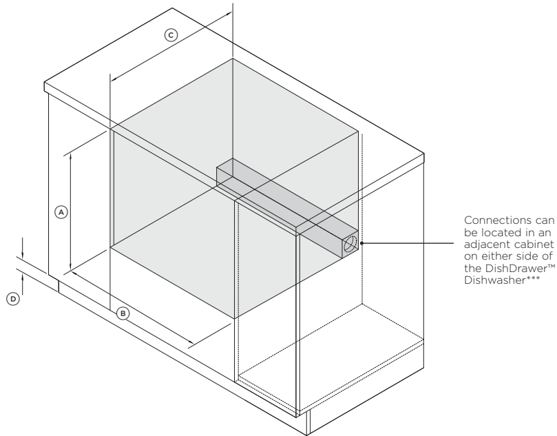
ISOMETRIC
